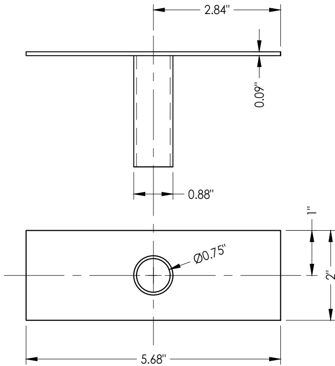
9 TUBE ANCHOR
