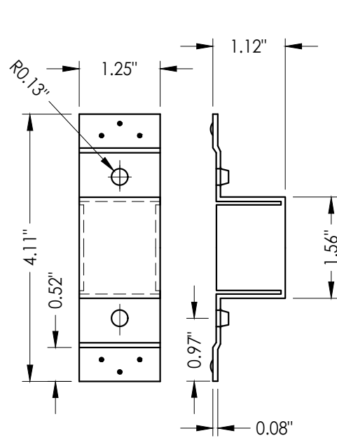
19 DEADBOLT STRIKE REINFORCEMENT
